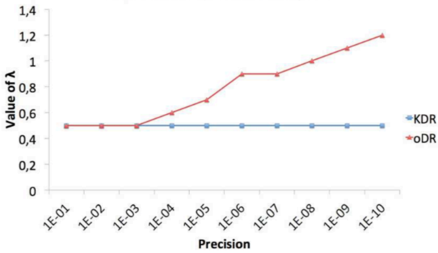
Required value of \lambda for convergence
